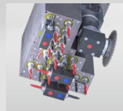
Standard drilling gear V18H6N 24 drilling spindles [High-Speed 7500] ▪ 18 vertical drilling spindles ▪ 6 horizontal drilling spindles (4X2Y) ▪ 1 grooving saw Ø 125 mm (0° / 90°)
