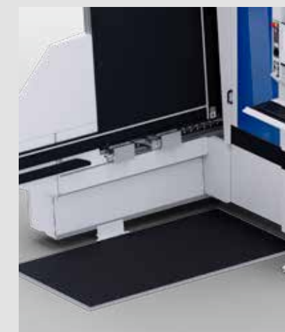
Safety concept with safety shut off mats The focus is on optimized and safe interaction between operator and machine. The infeed and outfeed are equipped with safety mats that are activated as soon as the machine operator steps on them. Thanks to the auto-quit feature, the process re-starts automatically when leaving the mat.
