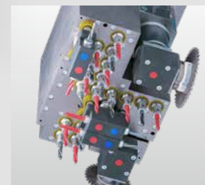
Optional drilling gear V17H6N2 23 drilling spindles [High-Speed 7500] ▪ 17 vertical drilling spindles ▪ 6 horizontal drilling spindles (4X2Y) ▪ 1 grooving saw Ø 125 mm (0° / 90°) ▪ 1 grooving saw Ø 100 mm
